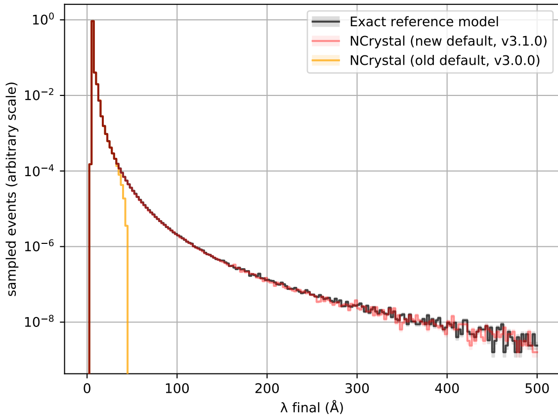
Sampling 1K He4 kernel with 5.0Å neutrons
