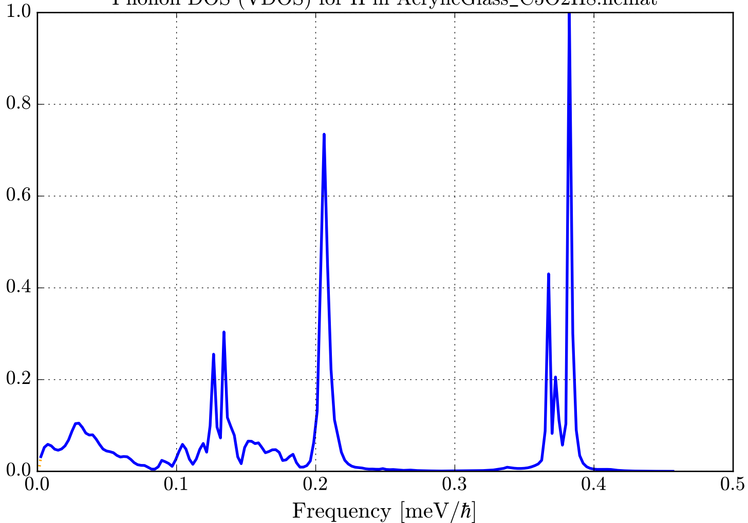
Phonon DOS (VDOS) for H in AcrylicGlass_C5O2H8.ncmat
