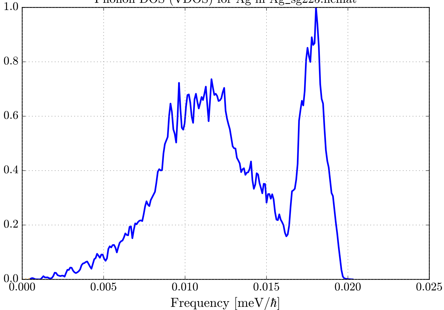
Phonon DOS (VDOS) for Ag in Ag_sg225.ncmat
