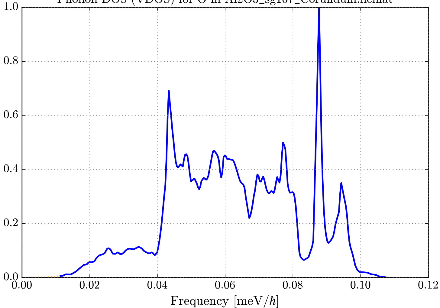
Phonon DOS (VDOS) for O in Al2O3_sg167_Corundum.ncmat
