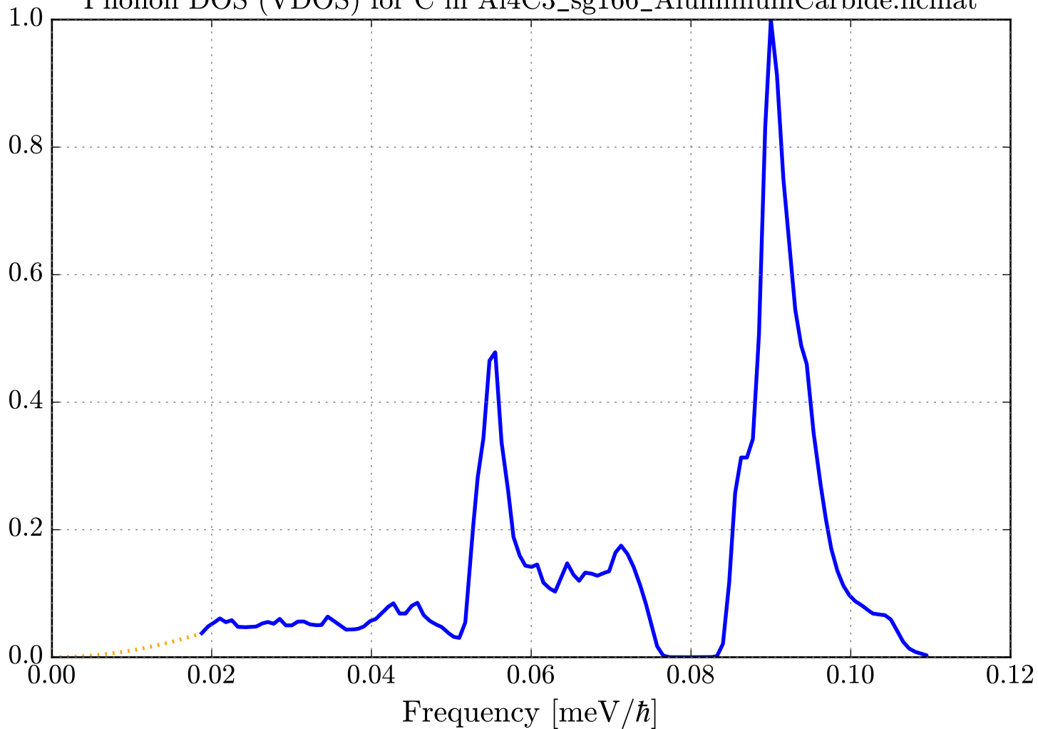
Phonon DOS (VDOS) for C in Al4C3_sg166_AluminiumCarbide.ncmat
