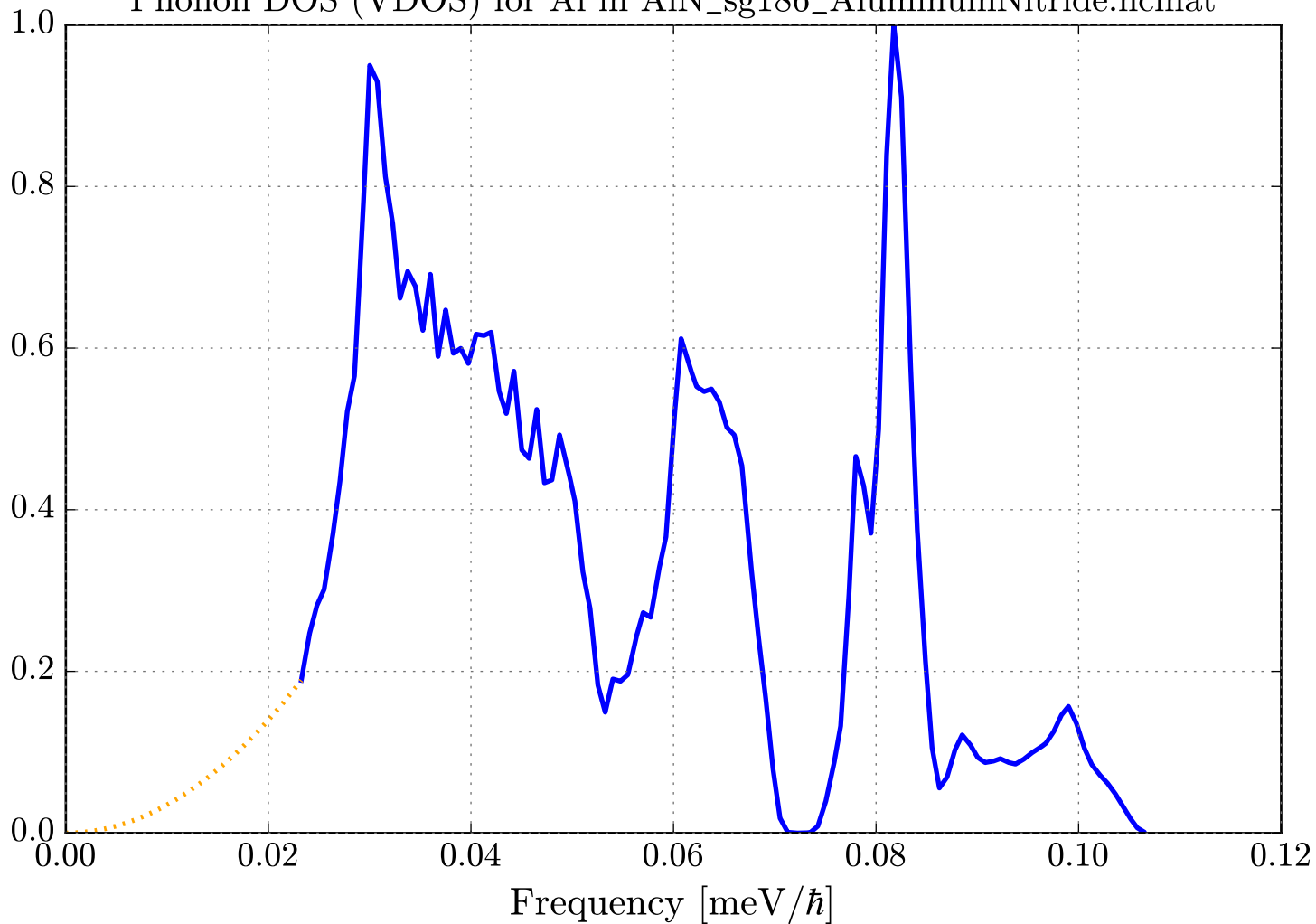
Phonon DOS (VDOS) for Al in AlN_sg186_AluminumNitride.ncmat
