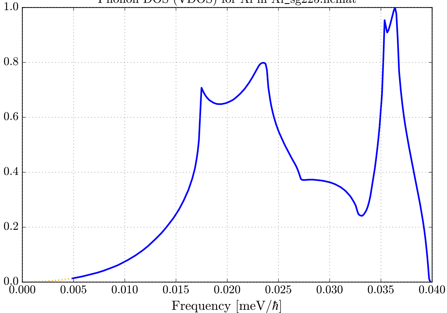
Phonon DOS (VDOS) for Al in Al_sg225.ncmat
