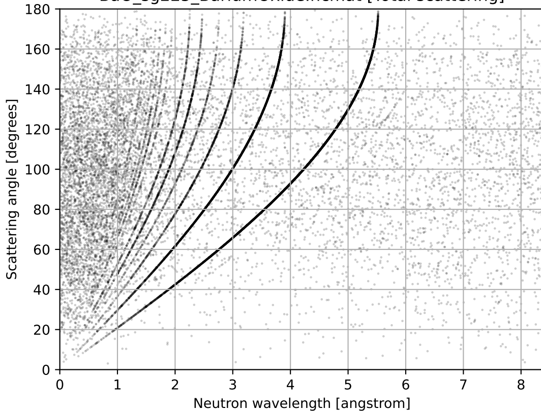
BaO_sg225_BariumOxide.ncmat [Total scattering]
