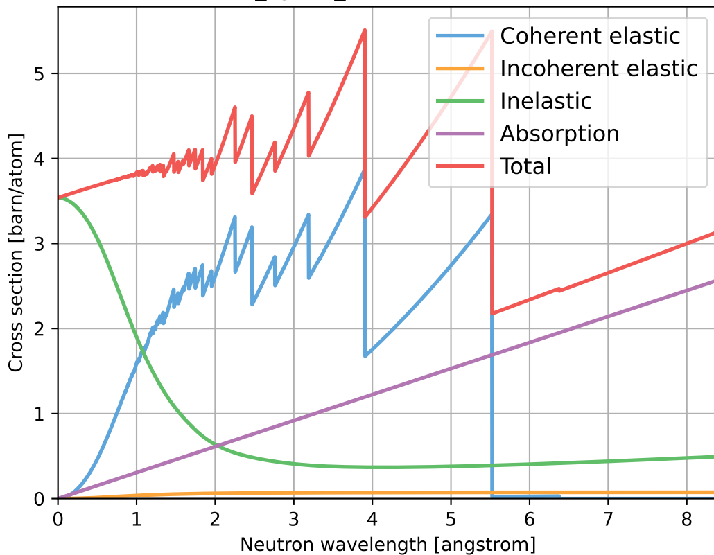
BaO_sg225_BariumOxide.ncmat
