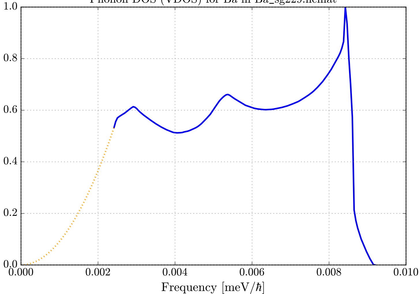
Phonon DOS (VDOS) for Ba in Ba_sg229.ncmat
