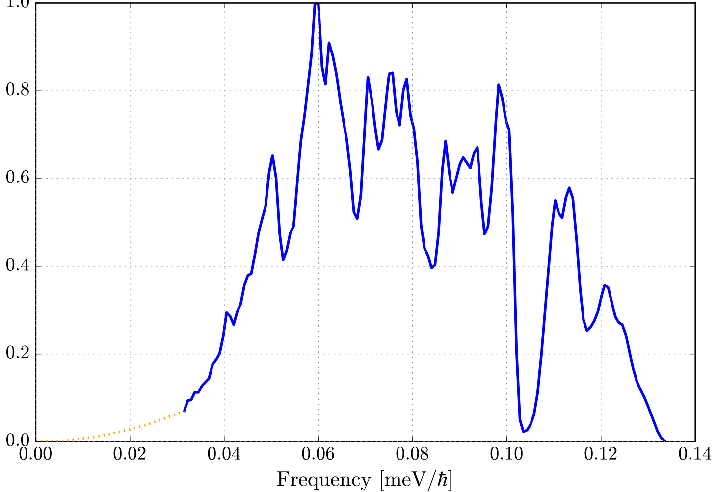
Phonon DOS (VDOS) for Be in Be 3 N 2 _sg206_BerylliumNitride.ncmat
