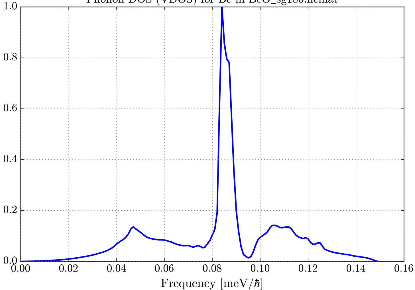
Phonon DOS (VDOS) for Be in BeO_sg186.ncmat
