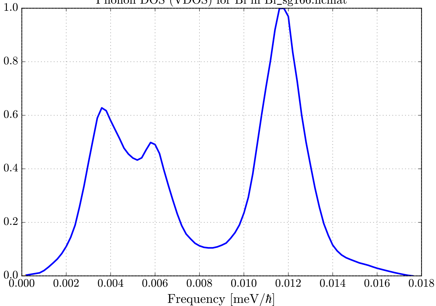
Phonon DOS (VDOS) for Bi in Bi_sg166.ncmat
