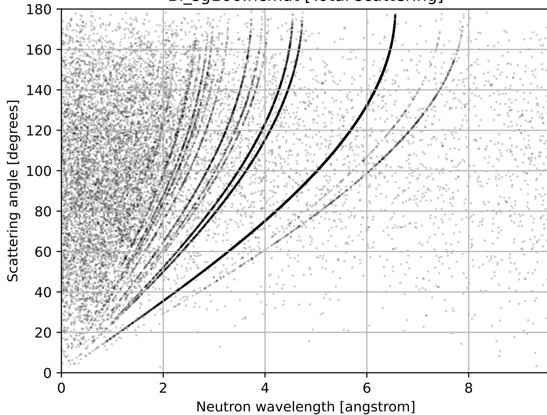
Bi_sg166.ncmat [Total scattering]
