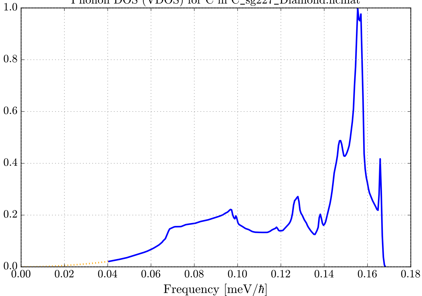
Phonon DOS (VDOS) for C in C_sg227_Diamond.ncmat
