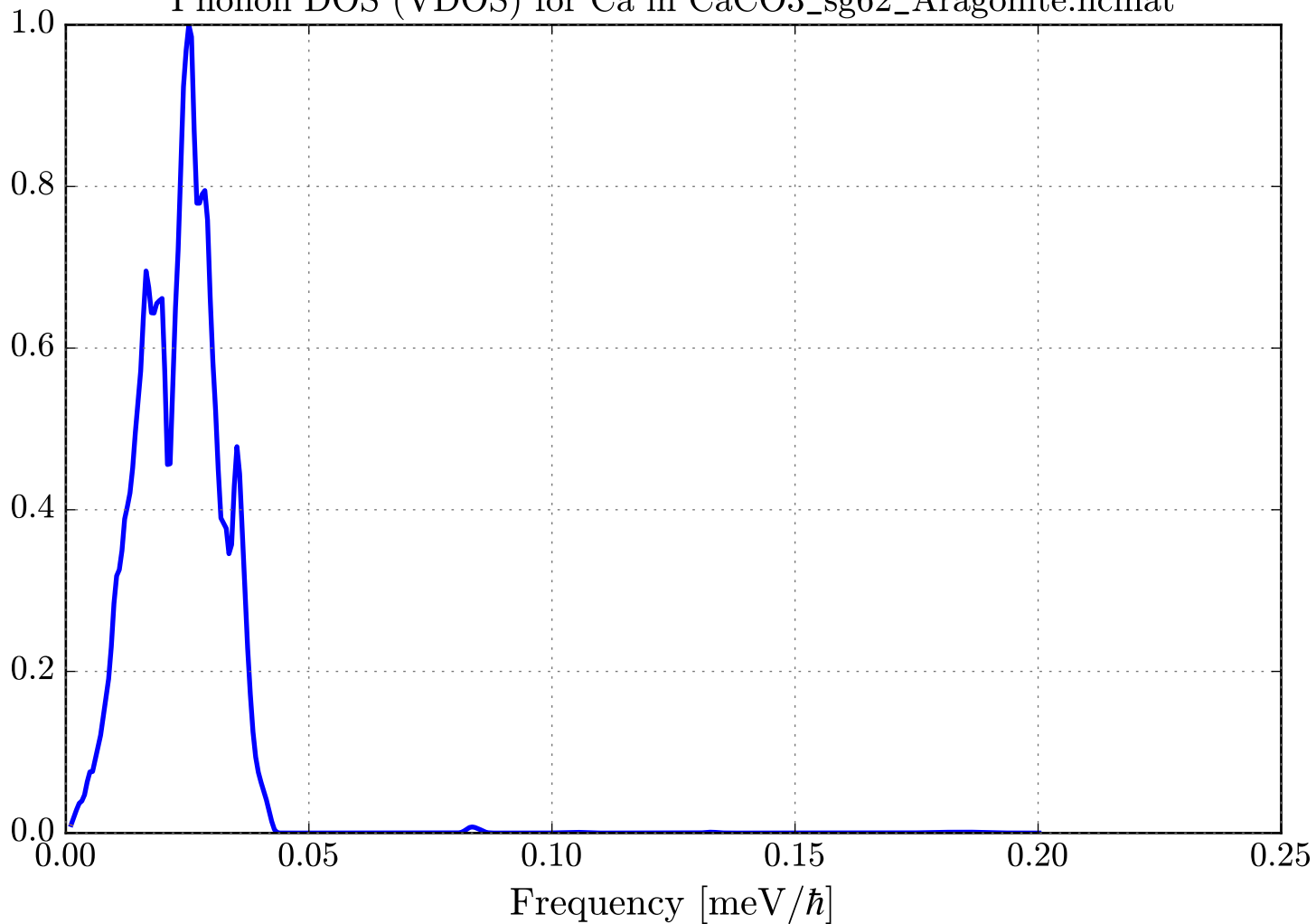
Phonon DOS (VDOS) for Ca in CaCO 3 _sg62_Aragonite.ncmat
