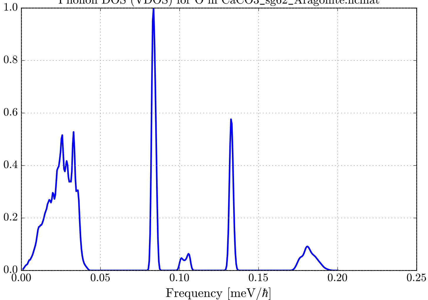
Phonon DOS (VDOS) for O in CaCO 3 _sg62_Aragonite.ncmat
