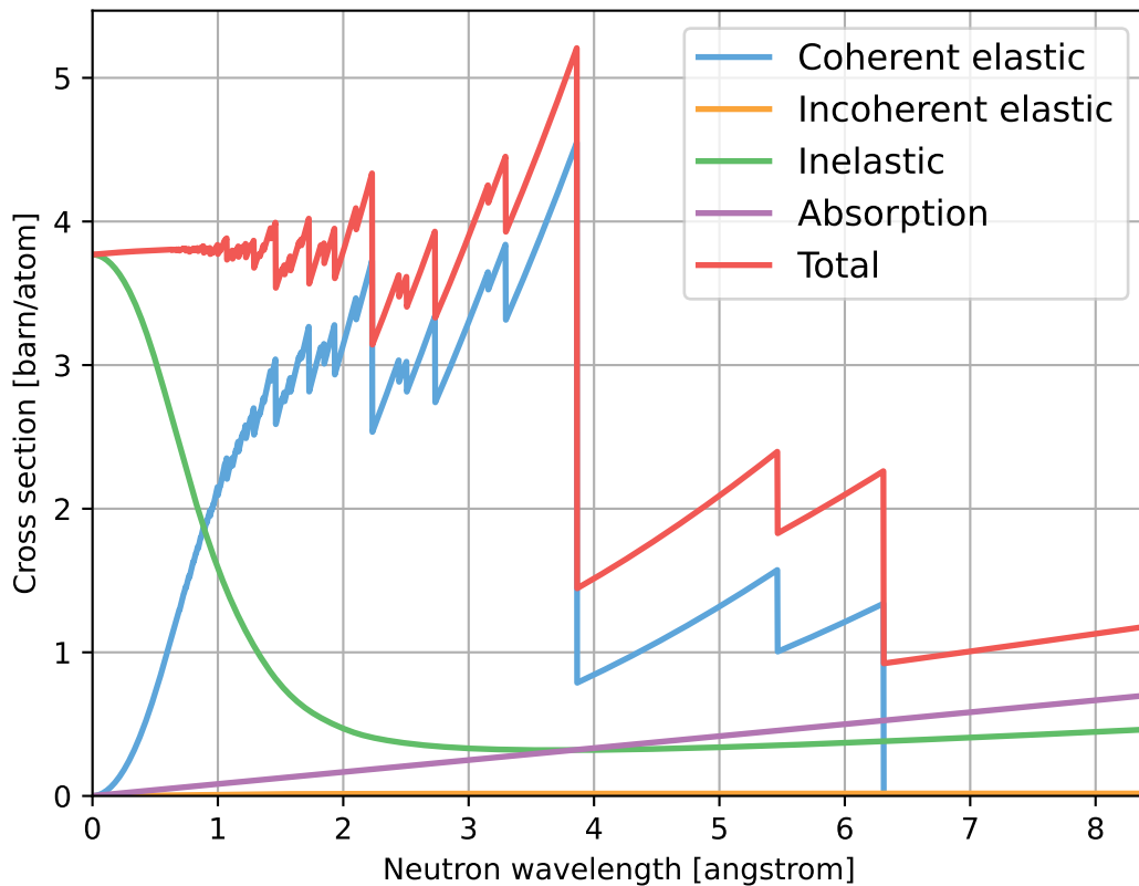
CaF2_sg225_CalciumFlouride.ncmat
