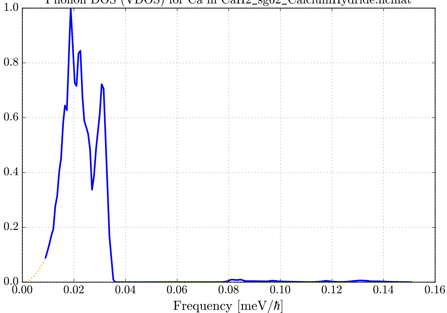
Phonon DOS (VDOS) for Ca in CaH2_sg62_CalciumHydride.ncmat
