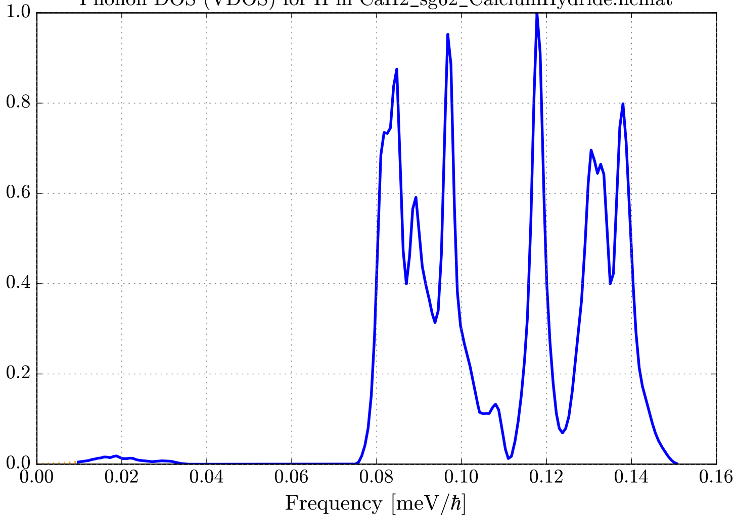
Phonon DOS (VDOS) for H in CaH2_sg62_CalciumHydride.ncmat
