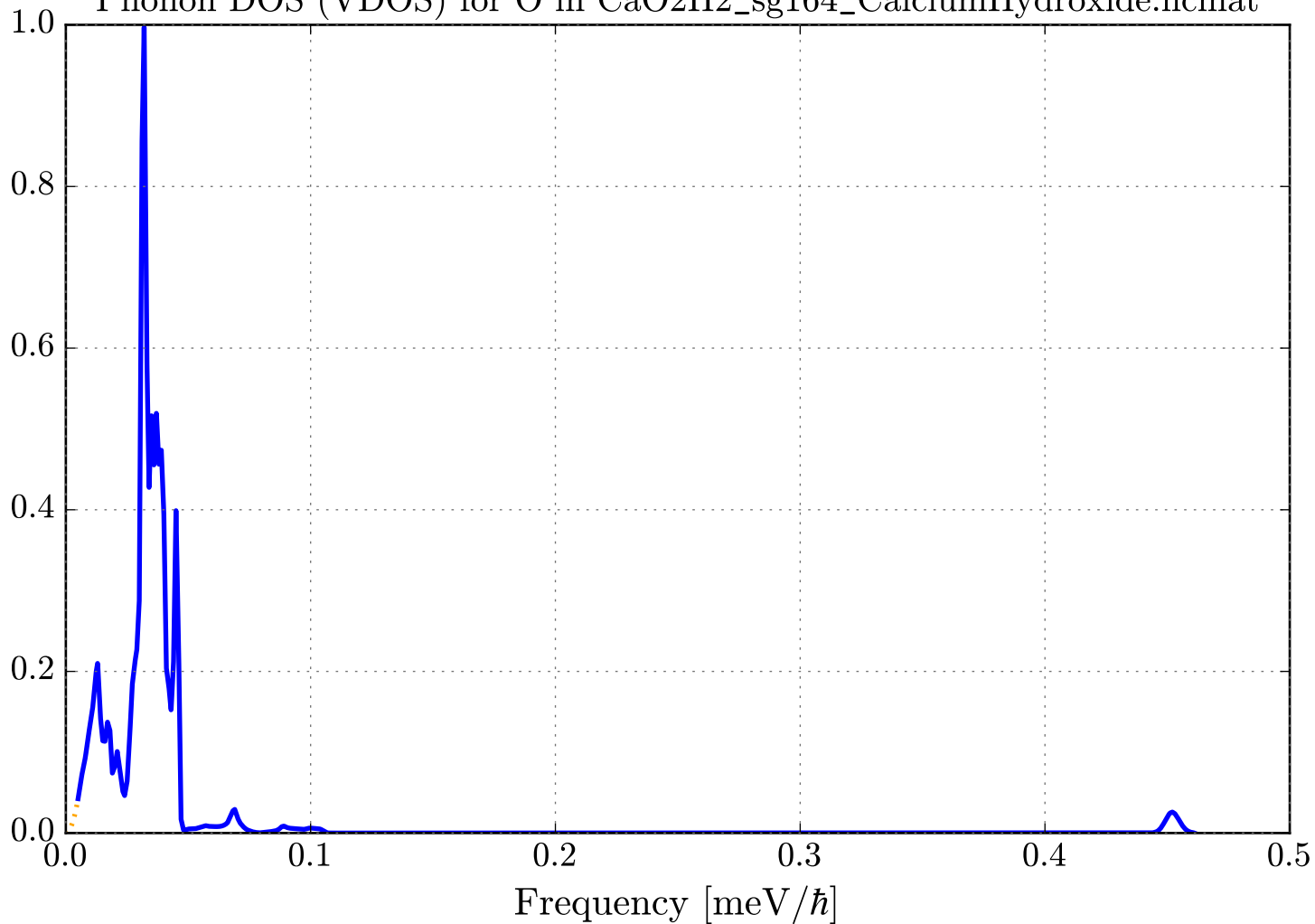
Phonon DOS (VDOS) for O in CaO2H2_sg164_CalciumHydroxide.ncmat
