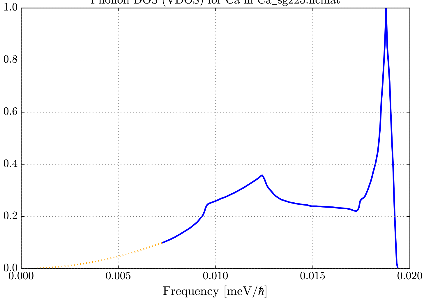
Phonon DOS (VDOS) for Ca in Ca_sg225.ncmat
