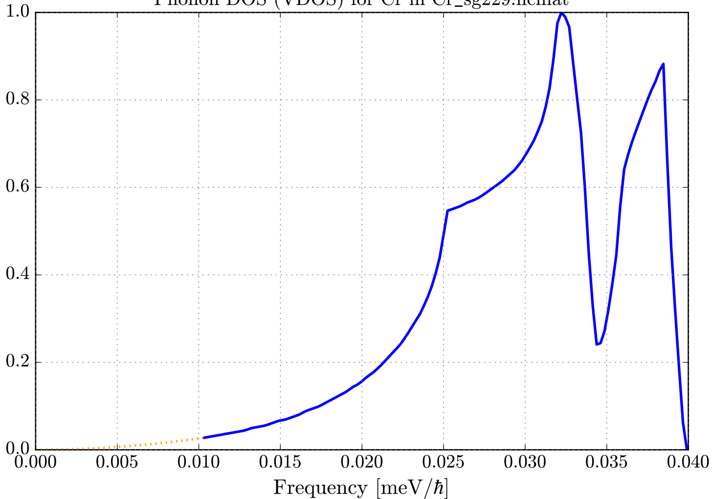
Phonon DOS (VDOS) for Cr in Cr_sg229.ncmat
