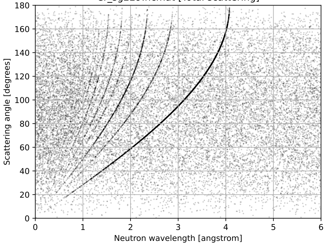
Cr_sg229.ncmat [Total scattering]
