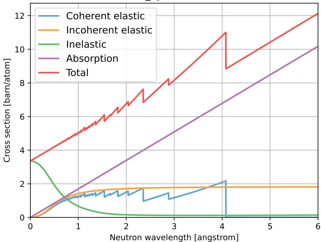
Cr_sg229.ncmat
