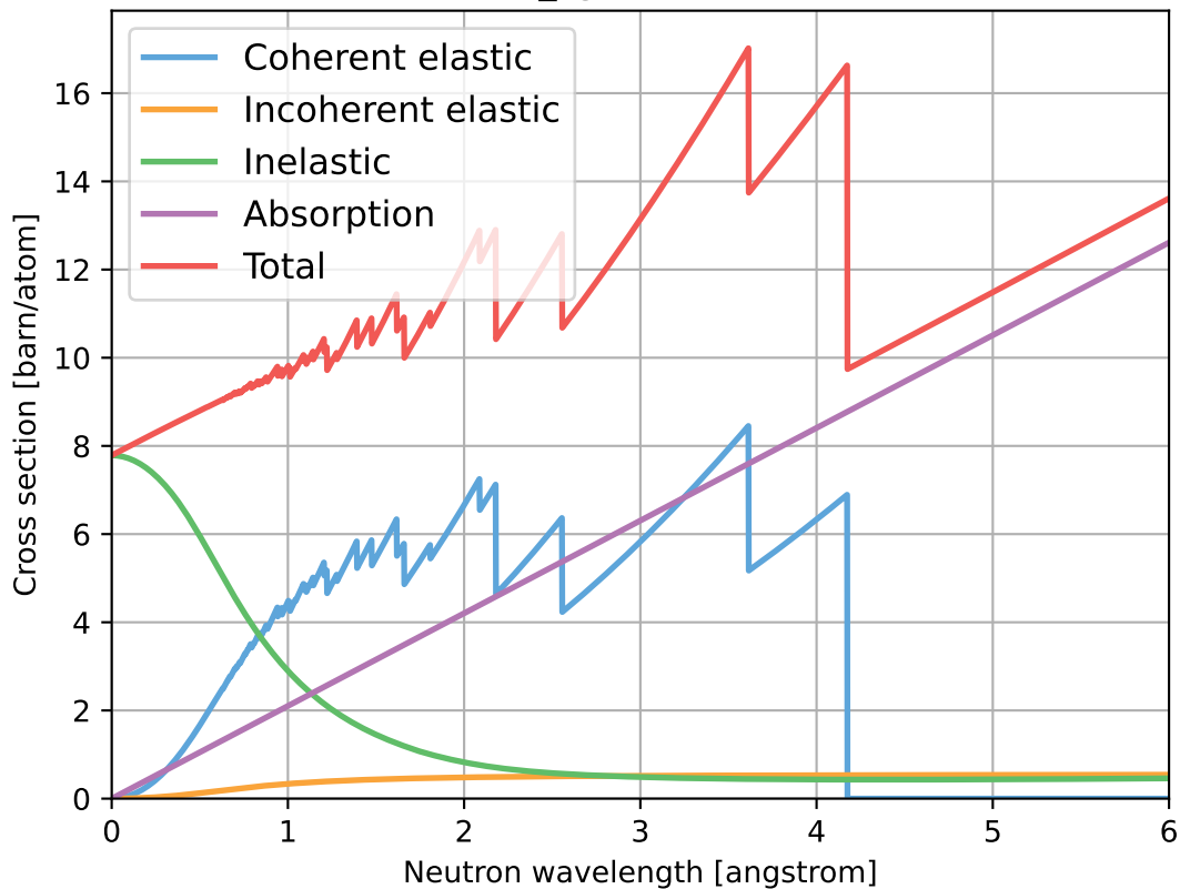
Cu_sg225.ncmat
