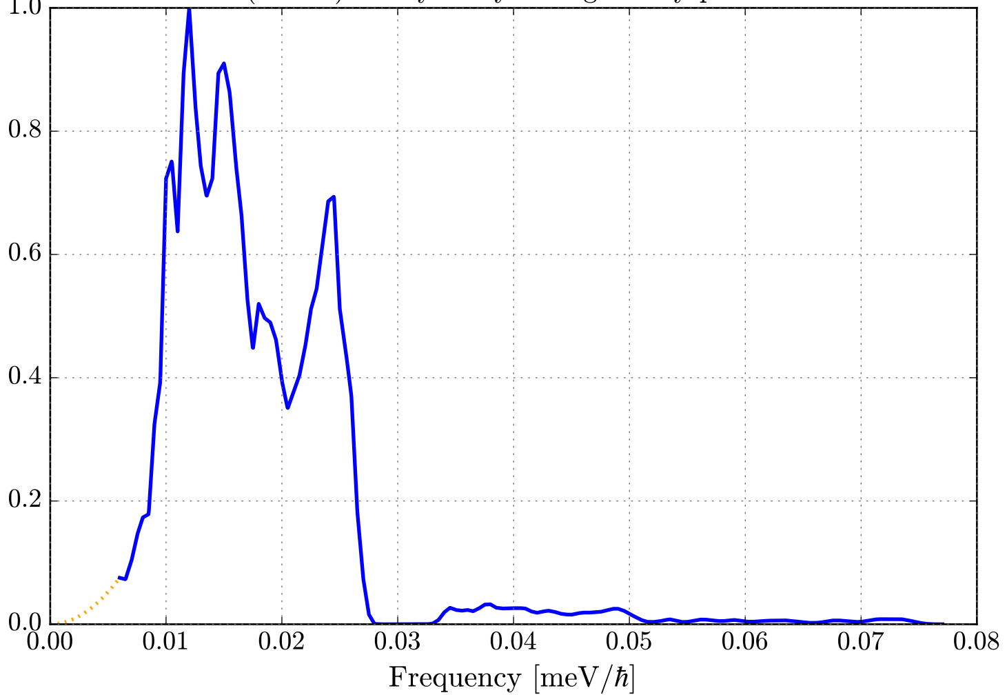
Phonon DOS (VDOS) for Dy in Dy2O3_sg206_DysprosiumOxide.ncmat
