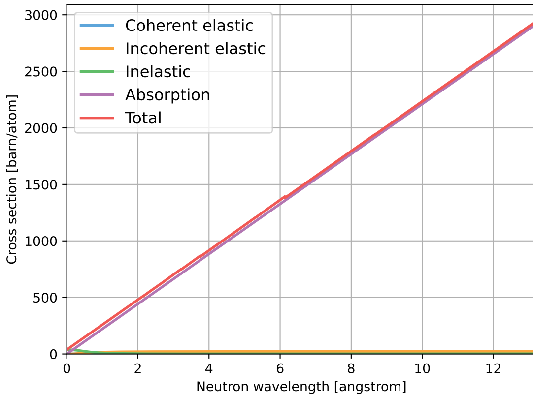
Dy2O3_sg206_DysprosiumOxide.ncmat
