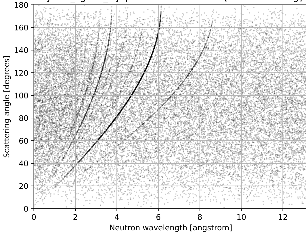
Dy2O3_sg206_DysprosiumOxide.ncmat [Total scattering]
