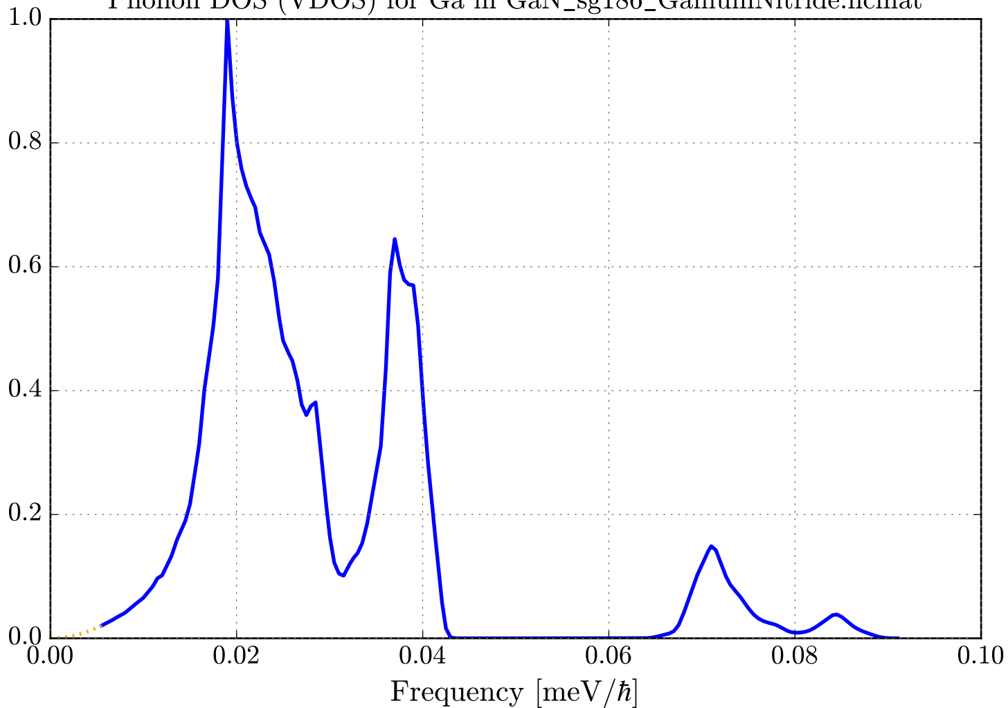
Phonon DOS (VDOS) for Ga in GaN_sg186_GalliumNitride.ncmat
