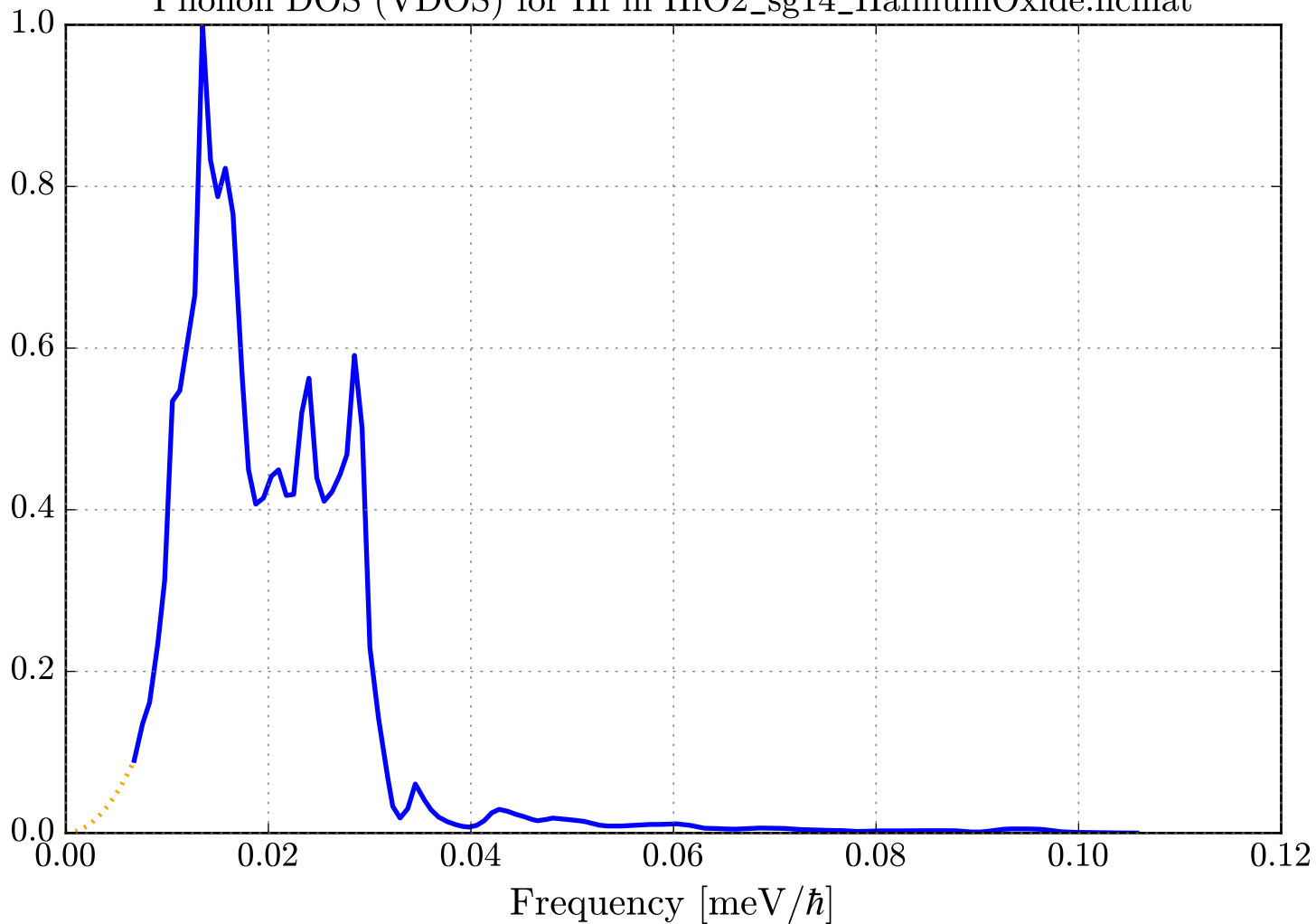
Phonon DOS (VDOS) for Hf in HfO2_sg14_HafniumOxide.ncmat
