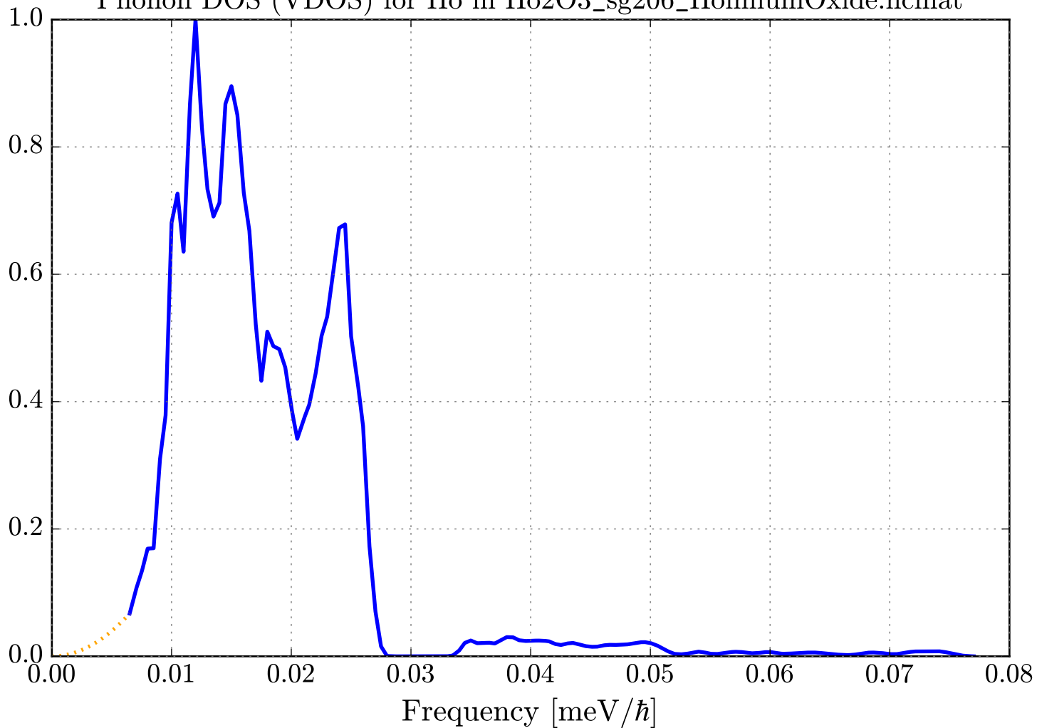
Phonon DOS (VDOS) for Ho in Ho2O3_sg206_HolmiumOxide.ncmat
