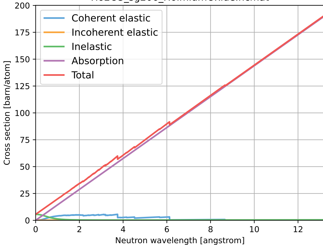
Ho2O3_sg206_HolmiumOxide.ncmat
