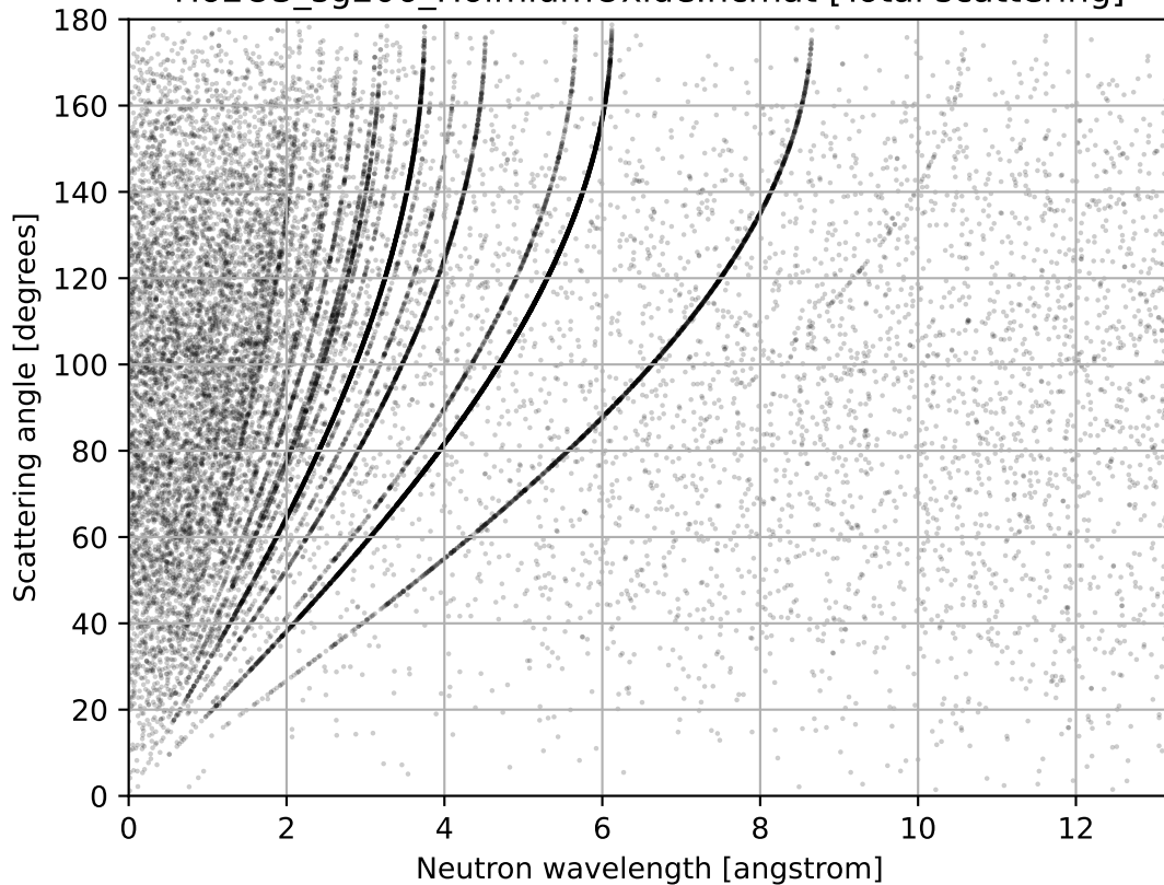
Ho2O3_sg206_HolmiumOxide.ncmat [Total scattering]
