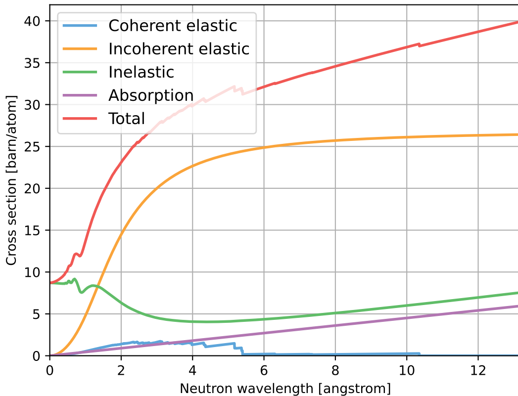
KOH_sg4_PotassiumHydroxide.ncmat
