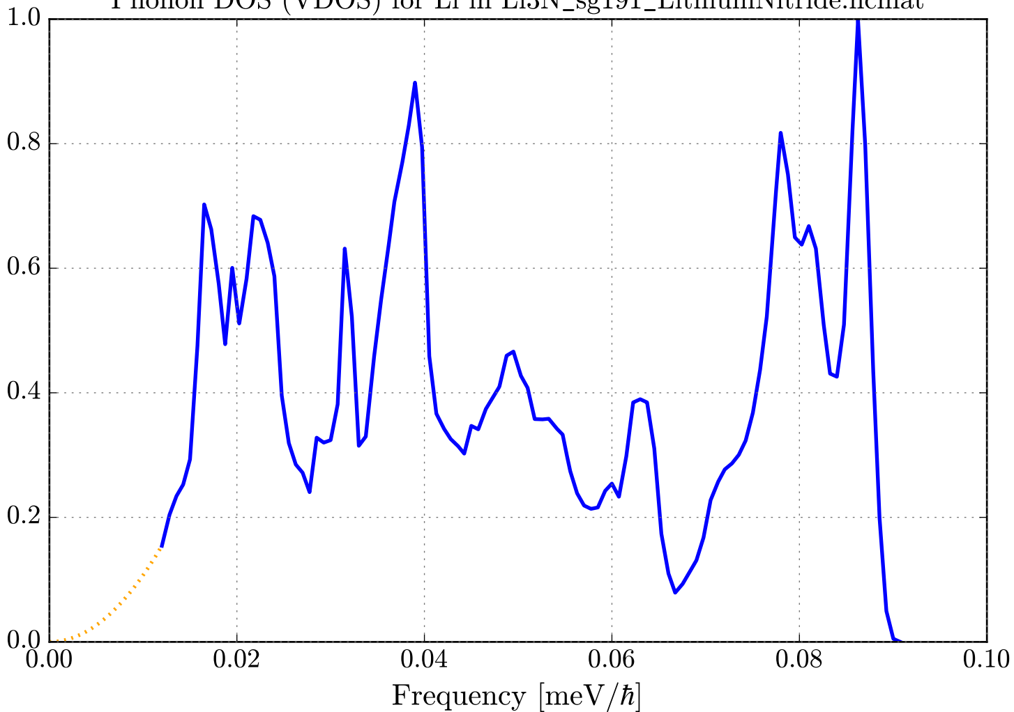
Phonon DOS (VDOS) for Li in Li3N_sg191_LithiumNitride.ncmat
