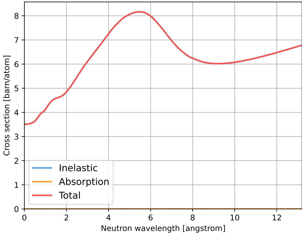
LiquidHeavyWaterD2O_T293.6K.ncmat
