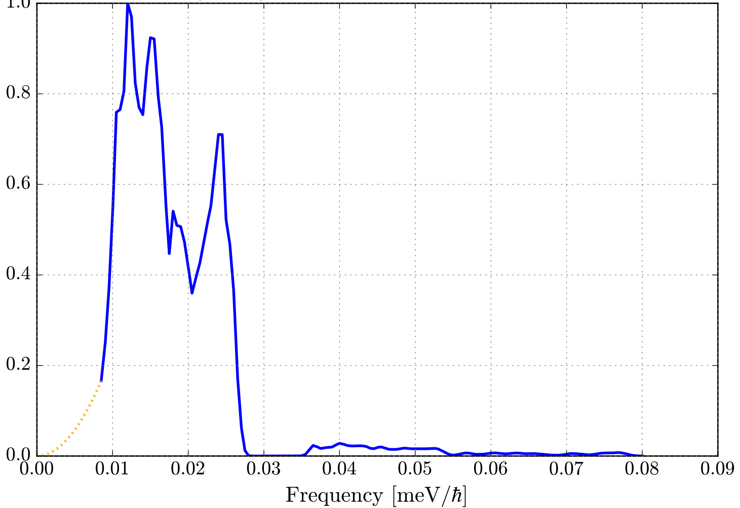
Phonon DOS (VDOS) for Lu in Lu2O3_sg206_LutetiumOxide.ncmat
