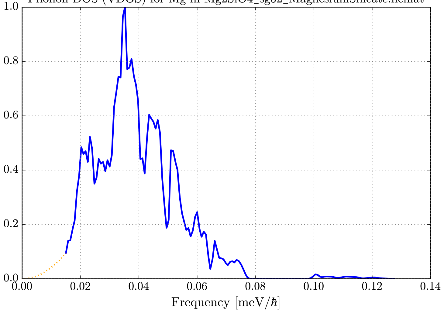
Phonon DOS (VDOS) for Mg in Mg 2 SiO 4 _sg62_MagnesiumSilicate.ncmat
