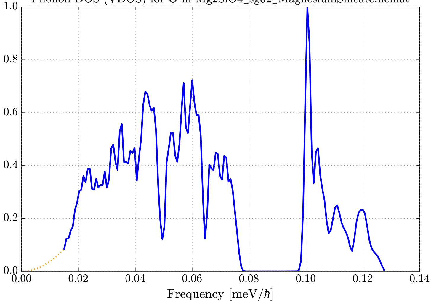
Phonon DOS (VDOS) for O in Mg 2 SiO 4 _sg62_MagnesiumSilicate.ncmat
