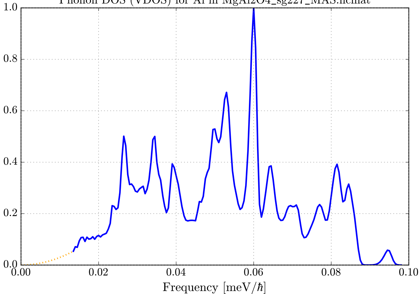
Phonon DOS (VDOS) for Al in MgAl2O4_sg227_MAS.ncmat
