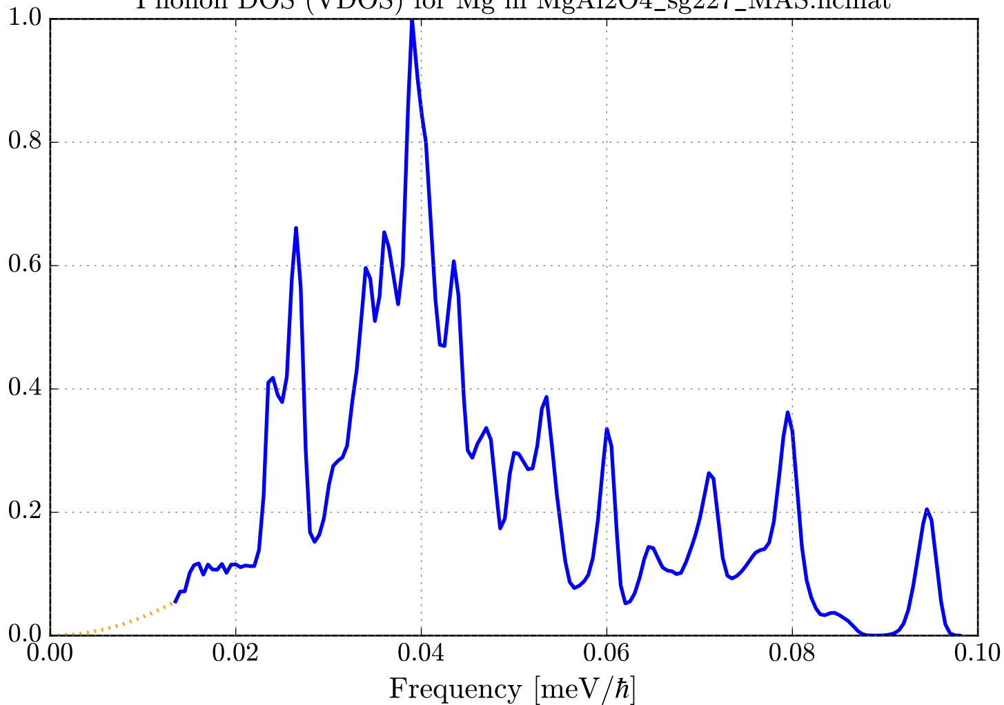
Phonon DOS (VDOS) for Mg in MgAl 2 O 4 _sg227_MAS.ncmat
