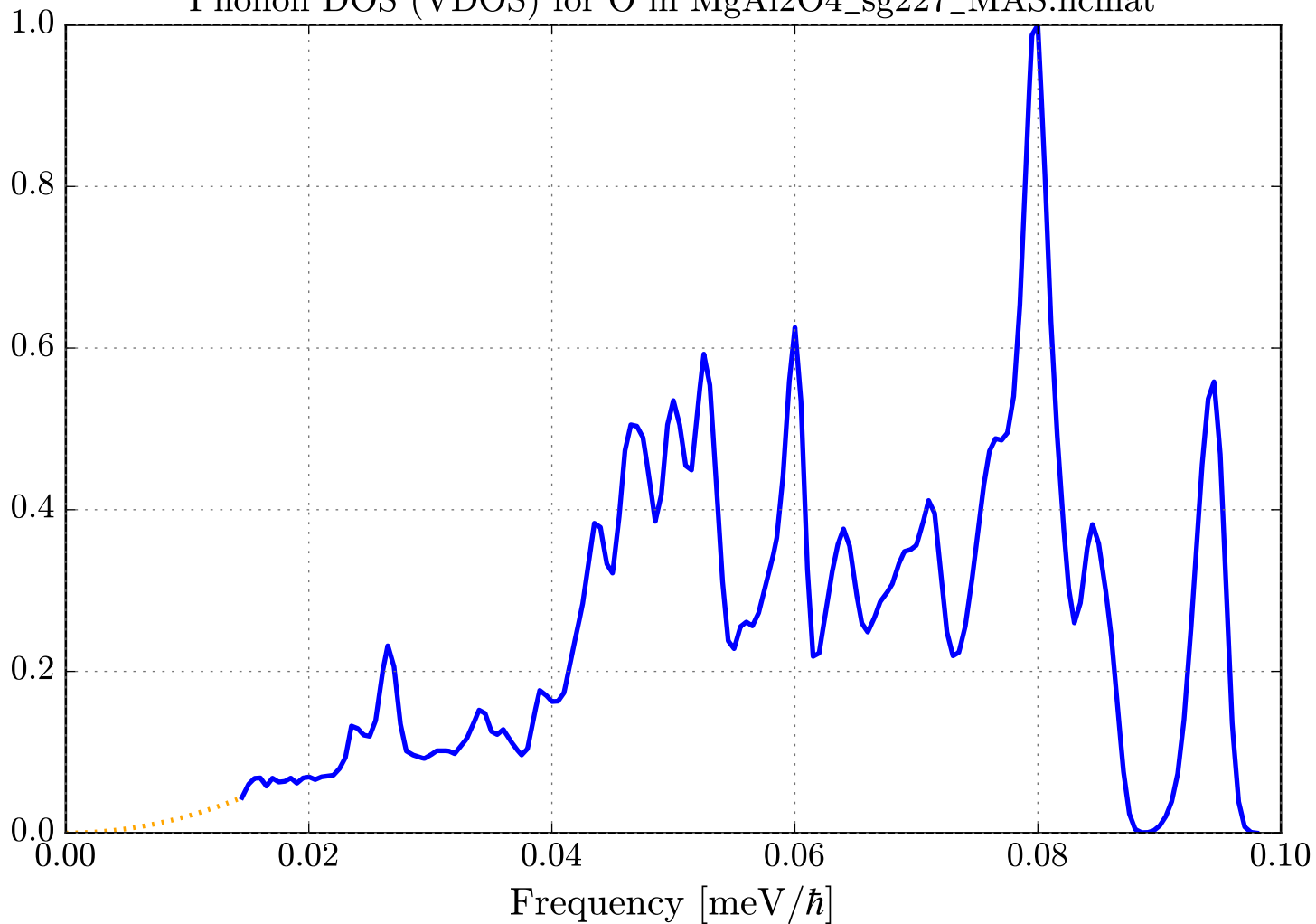
Phonon DOS (VDOS) for O in MgAl2O4_sg227_MAS.ncmat
