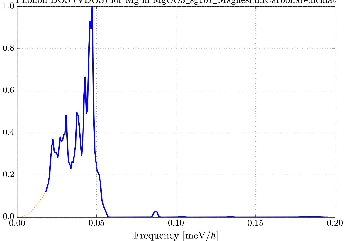
Phonon DOS (VDOS) for Mg in MgCO3_sg167_MagnesiumCarbonate.ncmat
