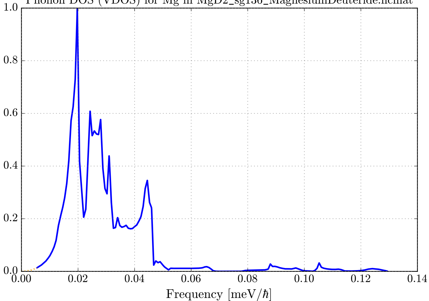
Phonon DOS (VDOS) for Mg in MgD2_sg136_MagnesiumDeuteride.ncmat
