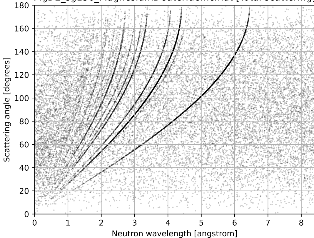
MgD2_sg136_MagnesiumDeuteride.ncmat [Total scattering]
