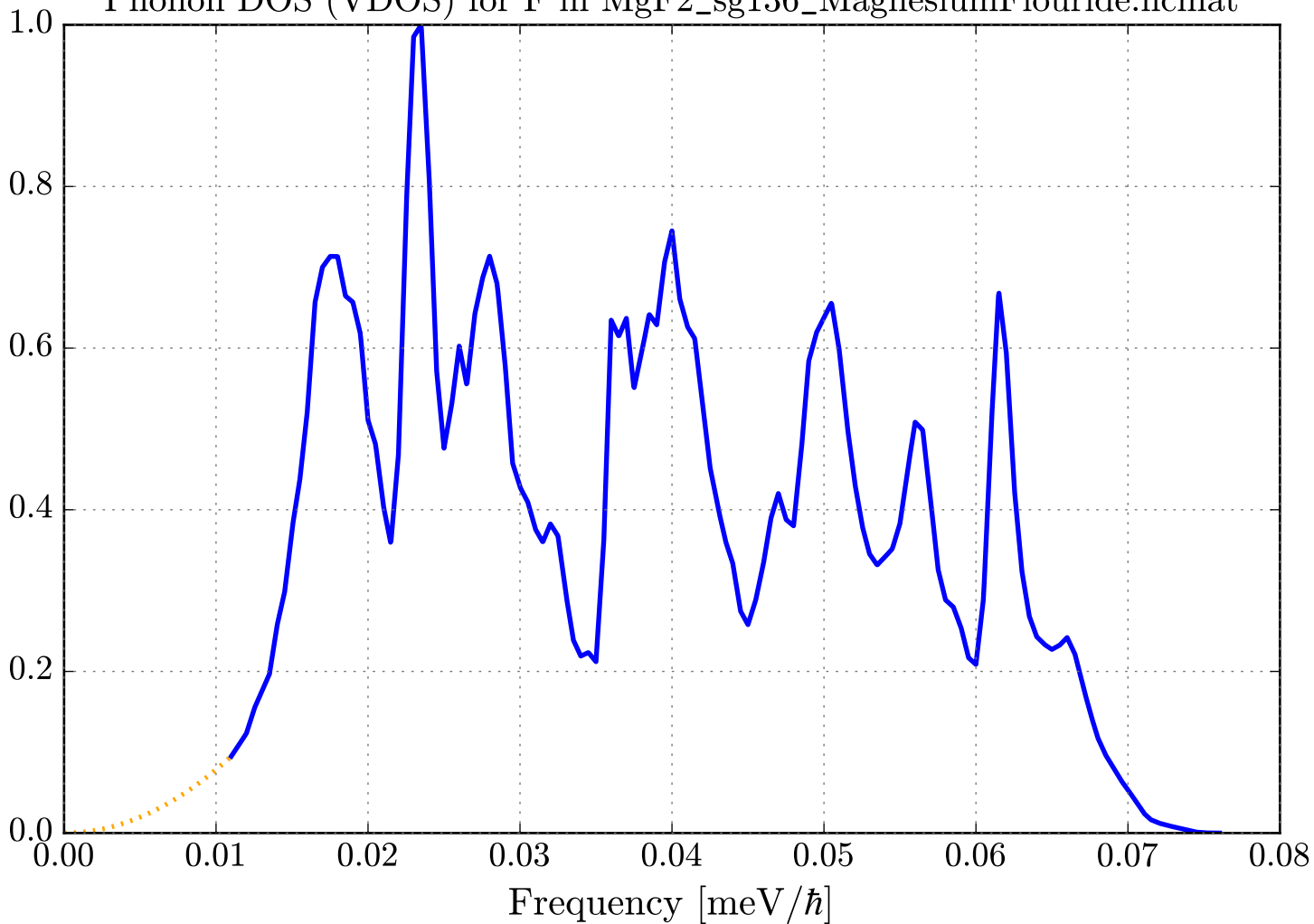
Phonon DOS (VDOS) for F in MgF2_sg136_MagnesiumFlouride.ncmat
