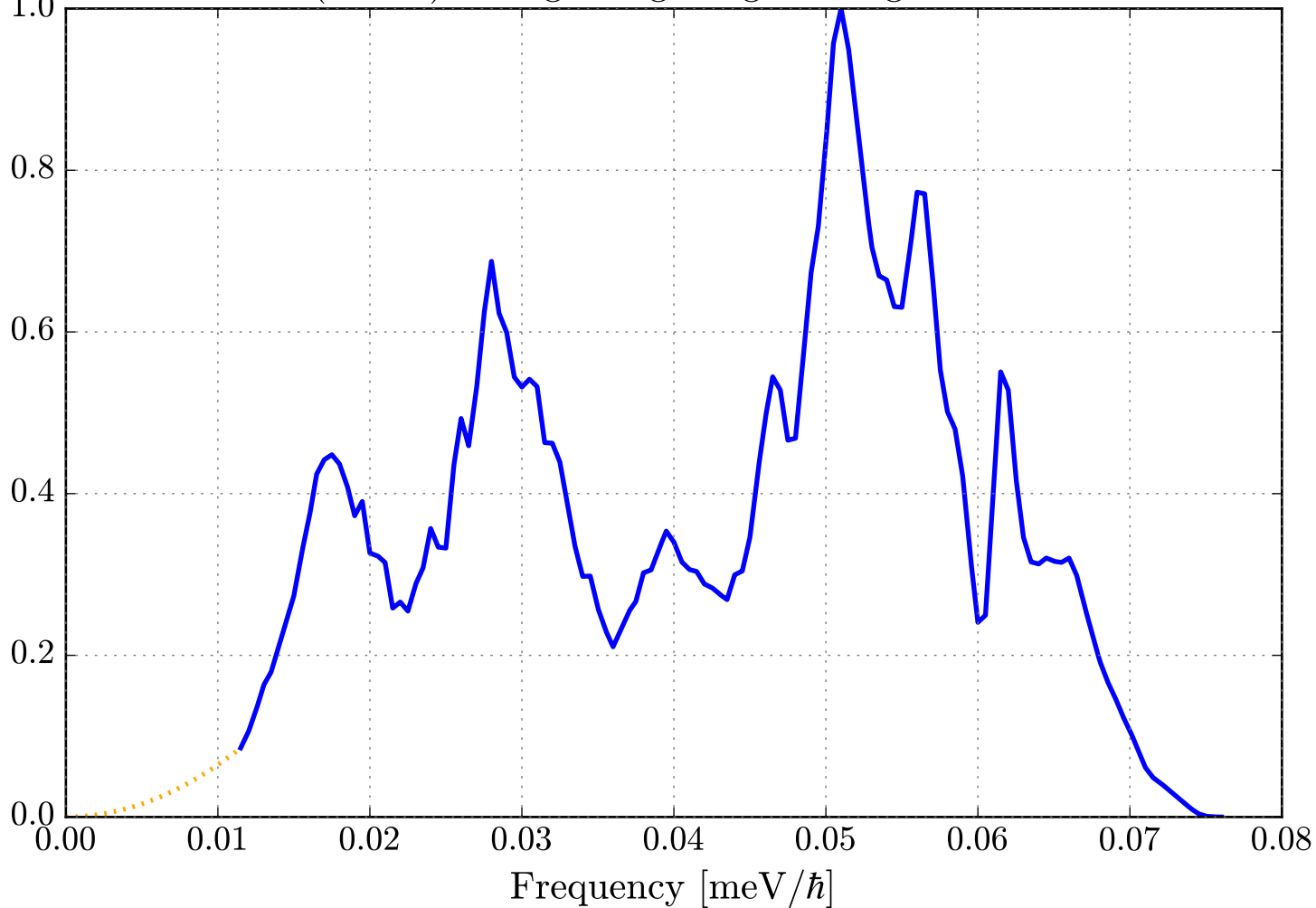
Phonon DOS (VDOS) for Mg in MgF2_sg136_MagnesiumFlouride.ncmat
