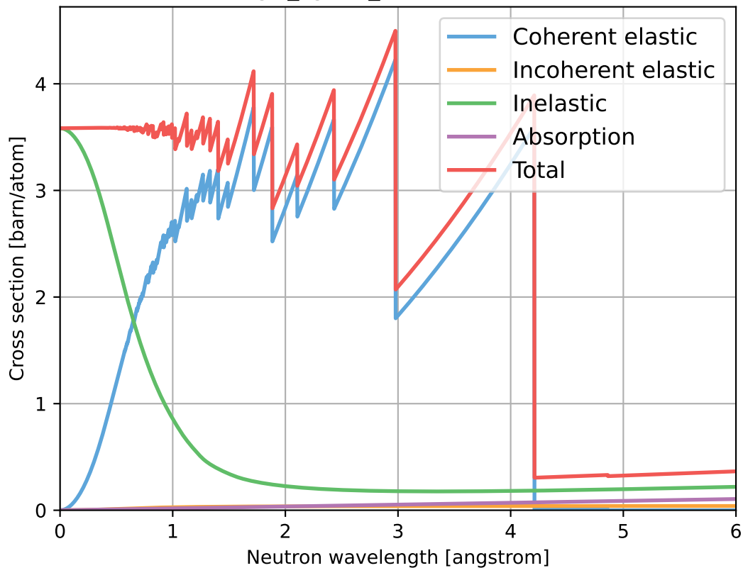
MgO_sg225_Periclase.ncmat
