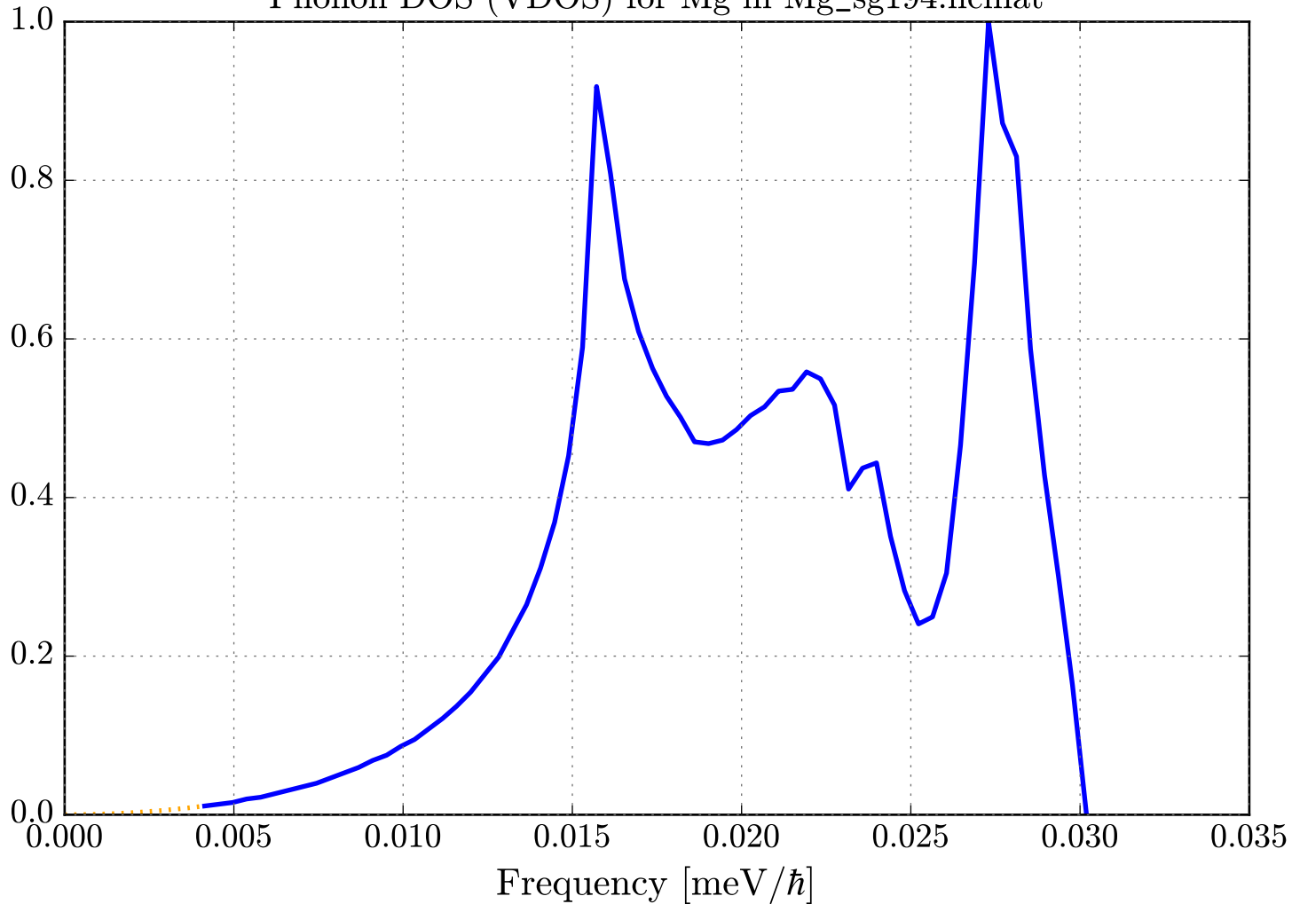
Phonon DOS (VDOS) for Mg in Mg_sg194.ncmat
