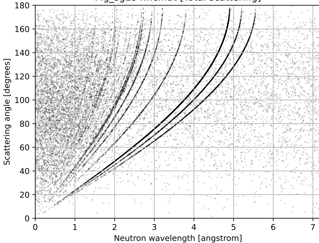
Mg_sg194.ncmat [Total scattering]
