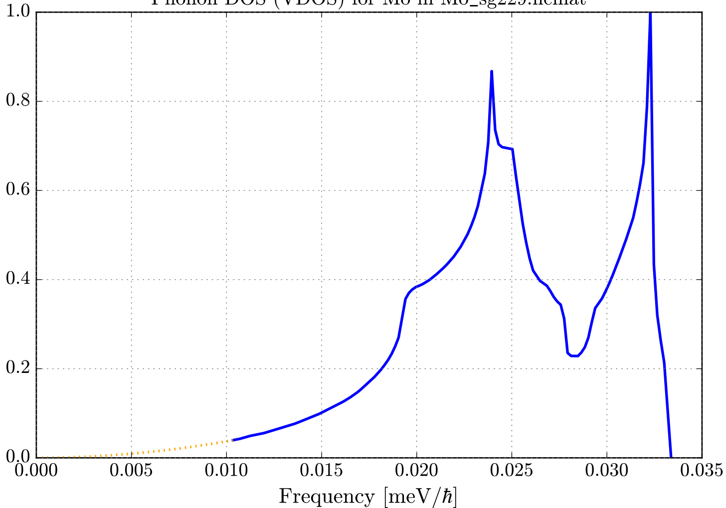
Phonon DOS (VDOS) for Mo in Mo_sg229.ncmat
