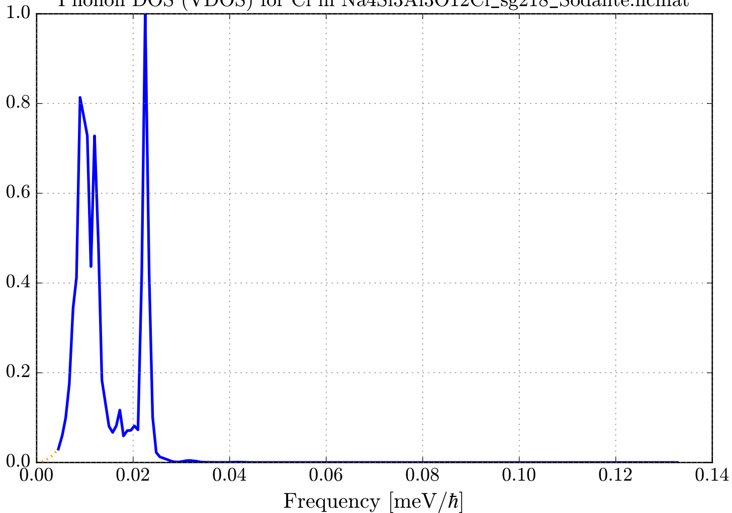
Phonon DOS (VDOS) for Cl in Na 4 Si 3 Al 3 O 12 Cl_sg218_Sodalite.ncmat
