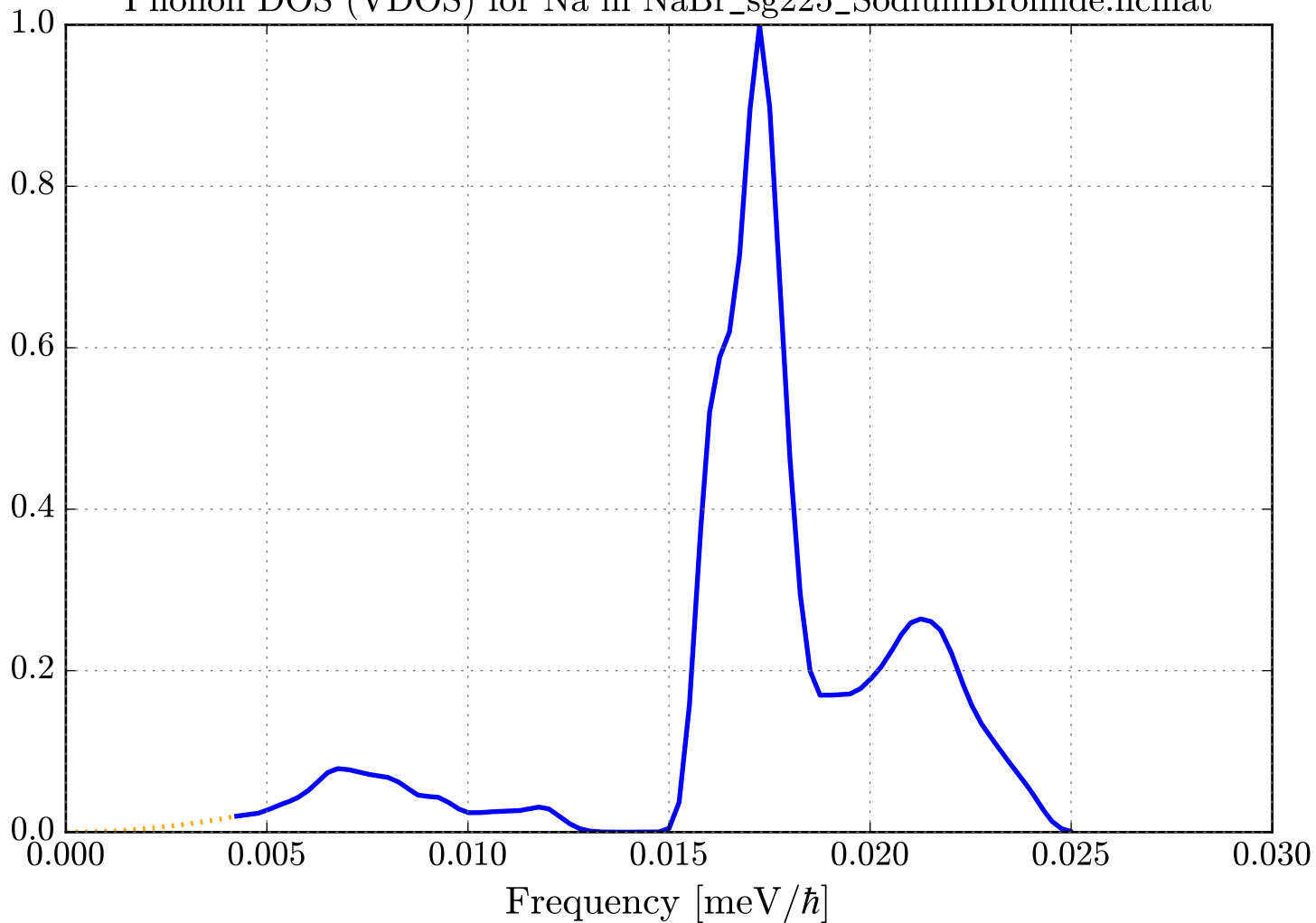
Phonon DOS (VDOS) for Na in NaBr_sg225_SodiumBromide.ncmat
